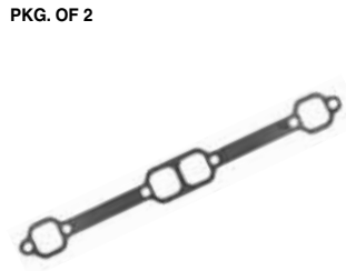
PKG. OF 2 18-2949 18-2949-9 ① EXHAUST MANIFOLD GASKET Replaces: Barr CHV-47-000 Use with: Manifold: 18-1997-1
