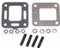
18-8514 EXHAUST ELBOW MOUNTING KIT Mercury Ford Small Block V8 302-351cu.in. (Models: 215, 225, 233, 255, 888), GM Small Block V8 305-351cu.in. (Models: 198,228,898) Used with: Riser: 18-1971 & 18-1978 (Not for Fresh Water/Closed Cooling Systems)
