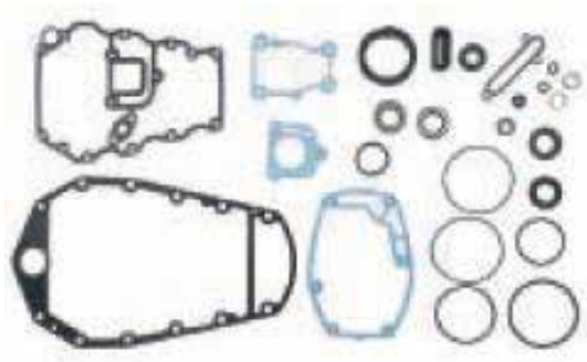
18-99093 GASKET SET Replaces: 67C-W0001-20 Fits: F30(2001), F40(2000-01), T25(2001)
