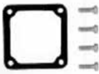
18-8500 EXHAUST ELBOW MOUNTING KIT Mercury 4 Cylinder 224cu.in. 3.7L (Models: 165, 170, 180, 190) Used with: Elbow/Reservoir: 18-1905
