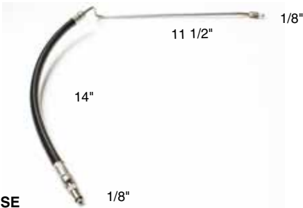
POWER TRIM HOSE Port • Connector to bottom of trim cylinder MCM 120-260 & BRAVO
